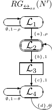
Fig. 5. The quotient reachability graph of N' = \text{Box}_{dtsd}(\overline{F}) for F = [(\{a\}, \rho) * ((\{b\}, \mathfrak{h}_k^1); (((\{c\}, \mathfrak{h}_l^0); (\{d\}, \theta)_1) || ((\{c\}, \mathfrak{h}_m^0); (\{d\}, \theta)_2))) * \text{Stop}]
