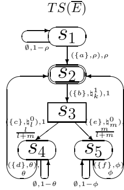
Fig. 1. The transition system of \overline{E} for E = [(\{a\}, \rho) * ((\{b\}, \mathfrak{h}_k^1); (((\{c\}, \mathfrak{h}_l^0); (\{d\}, \theta)) \square ((\{e\}, \mathfrak{h}_m^0); (\{f\}, \phi)))) * \mathbf{Stop}]
