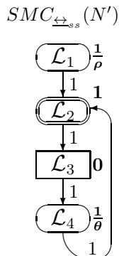
Fig. 7. The quotient underlying SMC of N' = \text{Box}_{\text{dtsd}}(\bar{F}) for F = [(\{a\}, \rho) * ((\{b\}, \mathfrak{h}_k^1); ((\{c\}, \mathfrak{h}_l^0); (\{d\}, \theta)_1) \parallel ((\{c\}, \mathfrak{h}_m^0); (\{d\}, \theta)_2))] * \text{Stop}
