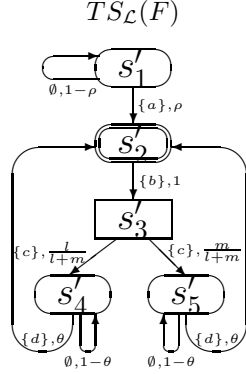
Fig. 3. The multi-action transition system of \overline{F} for F = [(\{a\}, \rho) * ((\{b\}, \mathbb{1}_k^1); (((\{c\}, \mathbb{1}_l^0); (\{d\}, \theta)_1) \parallel ((\{c\}, \mathbb{1}_m^0); (\{d\}, \theta)_2)))] * \text{Stop}
