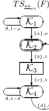
Fig. 4. The quotient transition system of \overline{F} for F = [(\{a\}, \rho) * ((\{b\}, \mathfrak{h}_k^1); (((\{c\}, \mathfrak{h}_l^0); (\{d\}, \theta)_1)[((\{c\}, \mathfrak{h}_m^0); (\{d\}, \theta)_2)) * \text{Stop}]
