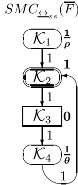
Fig. 6. The quotient underlying SMC of \overline{F} for F = [(\{a\}, \rho) * ((\{b\}, \mathfrak{h}_k^1); (((\{c\}, \mathfrak{h}_l^0); (\{d\}, \theta)_1)[((\{c\}, \mathfrak{h}_m^0); (\{d\}, \theta)_2)))] * \text{Stop}
