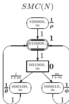
Fig. 2. The underlying SMC of N = Box_{dtsd}(\bar{E}) for E = [(\{a\}, \rho) * ((\{b\}, \natural_k^1); (((\{c\}, \natural_l^0); (\{d\}, \theta)) [((\{e\}, \natural_m^0); (\{f\}, \phi)))) * Stop]
