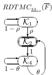
Fig. 9. The reduced quotient DTMC of \bar{F} for F = [(\{a\}, \rho) * ((\{b\}, \mathfrak{h}_k^1); (((\{c\}, \mathfrak{h}_i^0); (\{d\}, \theta)_1)[(\{c\}, \mathfrak{h}_m^0); (\{d\}, \theta)_2)) * \text{Stop}]
