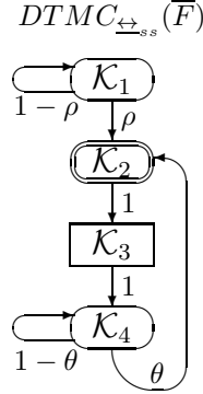
Fig. 8. The quotient DTMC of \bar{F} for F = [(\{a\}, \rho) * ((\{b\}, \mathfrak{h}_k^1); ((\{c\}, \mathfrak{h}_i^0); (\{d\}, \theta)_1)) \square ((\{c\}, \mathfrak{h}_m^0); (\{d\}, \theta)_2)) * \text{Stop}]
